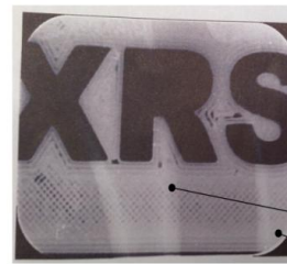
PLA based radio opaque XRS 80% infill / 5 mm thickness
